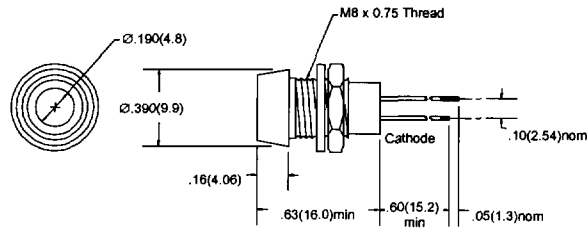
PMR200
