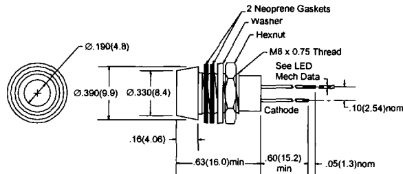
PMR200, Water-Tight
